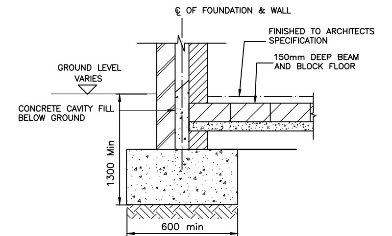
01,03 BEAM&BLOCK DETAIL 2 SCALE 1:20
