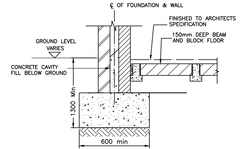
01,02 BEAM&BLOCK DETAIL 1 SCALE 1:20
