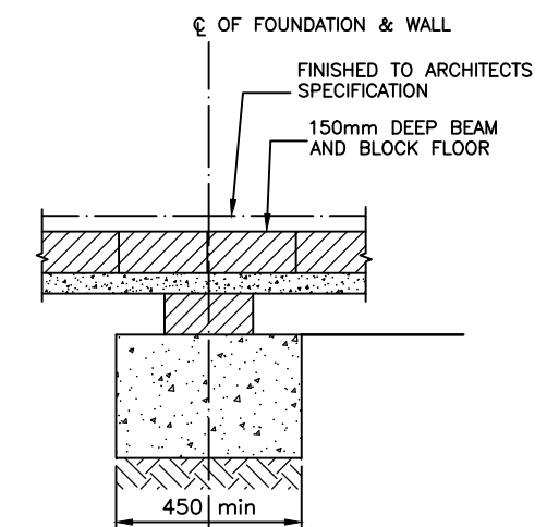
01,04 BEAM&BLOCK DETAIL 3 SCALE 1:20
